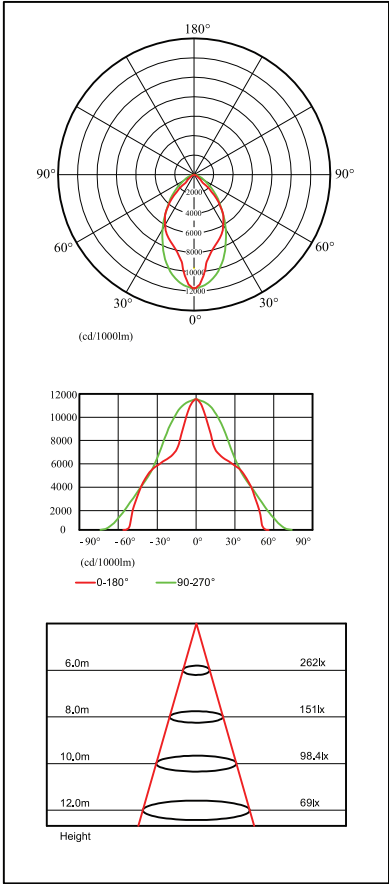
Beam angle 60°
